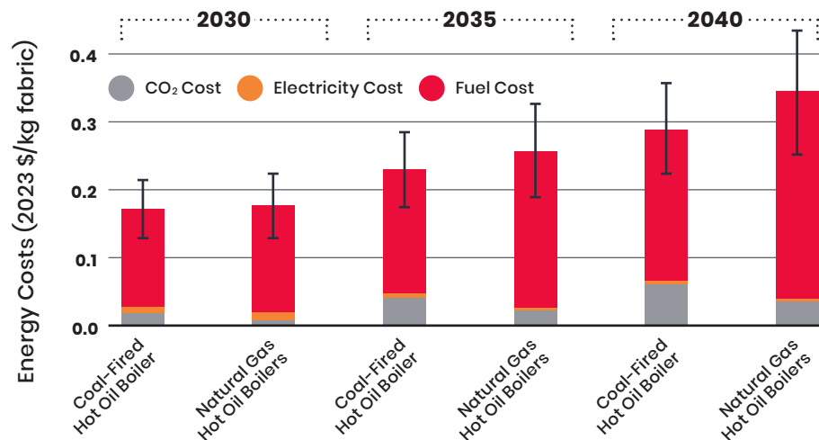
FIGURE 3.2.18: ENERGY COSTS OF COAL HOT OIL BOILERS VS. NATURAL GAS HOT OIL BOILERS IN A TYPICAL WET-PROCESSING FACILITY IN CHINA
