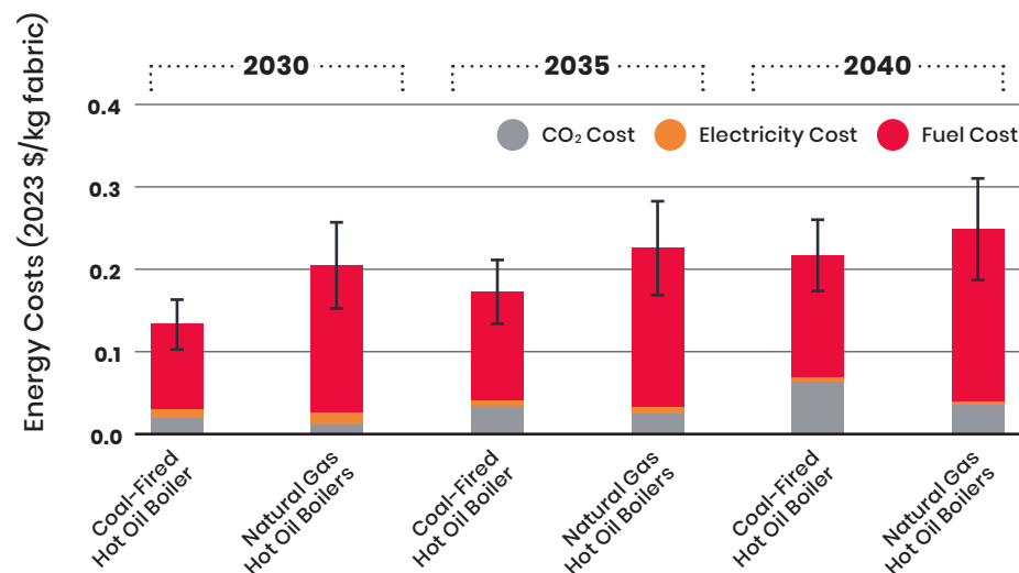
FIGURE 3.6.11. ENERGY COSTS OF COAL HOT OIL BOILERS VS. NATURAL GAS HOT OIL BOILERS IN A TYPICAL WET-PROCESSING FACILITY IN INDONESIA
