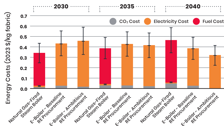
FIGURE 3.5.2: ENERGY COSTS OF NATURAL GAS STEAM BOILERS VS. ELECTRIC STEAM BOILERS IN BANGLADESH, BASELINE AND AMBITIOUS RE PROCUREMENT PATHWAYS
