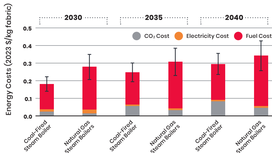
FIGURE 3.6.6. ENERGY COSTS OF COAL STEAM BOILERS VS. NATURAL GAS STEAM BOILERS IN A TYPICAL WET-PROCESSING FACILITY IN INDONESIA
