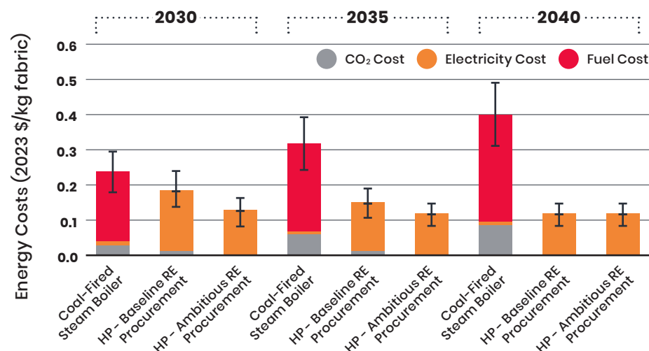
FIGURE 3.2.6: ENERGY COSTS OF COAL STEAM BOILERS VS. HEAT PUMPS, BASELINE AND AMBITIOUS RE PROCUREMENT PATHWAYS
