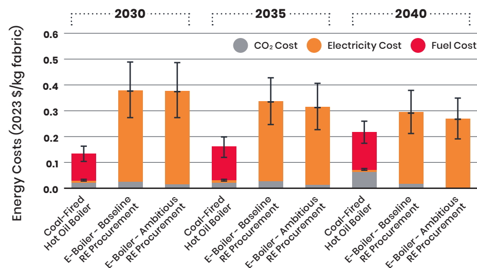
FIGURE 3.6.9: ENERGY COSTS OF COAL HOT OIL BOILERS VS. ELECTRIC HOT OIL BOILERS IN INDONESIA, BASELINE AND AMBITIOUS RE PROCUREMENT PATHWAYS
