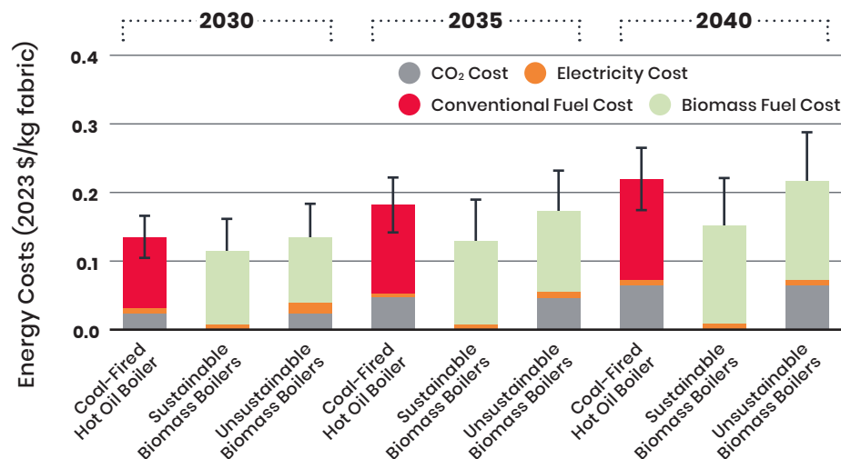
FIGURE 3.2.16: ENERGY COSTS OF COAL HOT OIL BOILERS VS. BIOMASS HOT OIL BOILERS (SUSTAINABLE AND UNSUSTAINABLE) IN A TYPICAL WET-PROCESSING FACILITY IN CHINA
