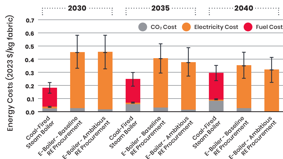
FIGURE 3.6.2. ENERGY COSTS OF COAL STEAM BOILERS VS. ELECTRIC STEAM BOILERS IN INDONESIA, BASELINE AND AMBITIOUS RE PROCUREMENT PATHWAYS
