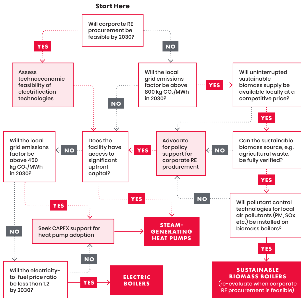
FIGURE ES5: DECISION TREE FOR TEXTILE FACILITIES IN THE STUDIED COUNTRIES SEEKING TO ADOPT LOW-CARBON THERMAL ENERGY TECHNOLOGIES
