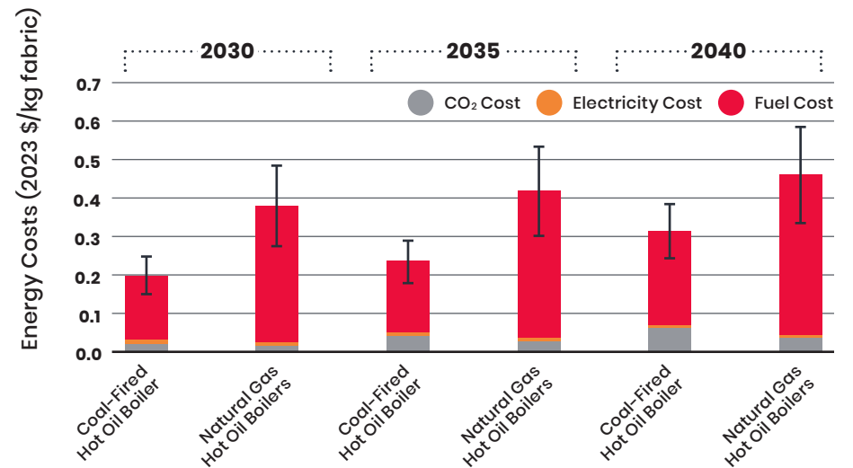
FIGURE 3.3.11: ENERGY COSTS OF COAL HOT OIL BOILERS VS. NATURAL GAS HOT OIL BOILERS IN A TYPICAL WET-PROCESSING FACILITY IN INDIA
